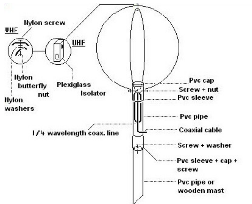
Fig 4 Practical building
