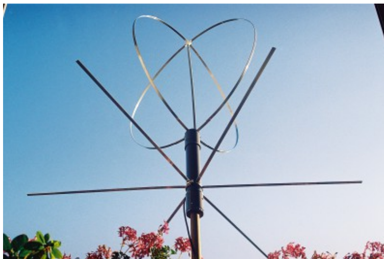
Fig. 5 "Eggbeater" VHF
